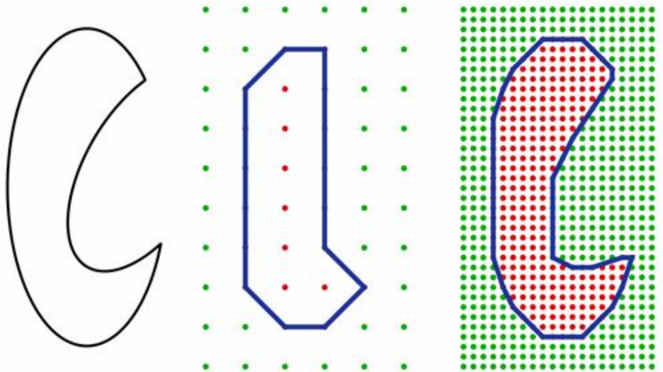
FIGURE 10.3. On the left, we outline a set S with boundary length of 91.0. In the middle, we show the relative convex hull's reconstruction of the boundary of S from a coarse sampling in blue. The length of the reconstructed boundary is 70.6. On the right, we show the relative convex hull's boundary reconstruction from a fine sampling, which has a length of 84.2. The length of the reconstructed boundary converges to the length of the boundary of S as the spacing between grid samples goes to zero.
