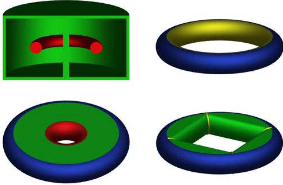
FIGURE 6.19. On the top left, we show sets R and G identical to the R and G in Figure 6.18. The tight hull of R relative to G is equal to R . We show the tight hull on the top right, with the boundary colored to indicate the amount of support at each point. The blue part of the boundary on the outer wall of the torus is fully supported, while the yellow part is only partially supported, because some sections at the yellow points are convex and others are concave. On the lower left, we show a candidate hull that minimizes slack but not unsupported slack. The red portion of the hull boundary is unsupported. The green portion is also unsupported, but it is developable, so its slack is zero and it does not contribute unsupported slack. We show another candidate hull on the bottom right. Part of the hull's slack is supported on the four yellow arcs, but the support from those arcs is less than the support from the inner wall of the torus in the tight hull on the top right, so this candidate is not a tight hull.
