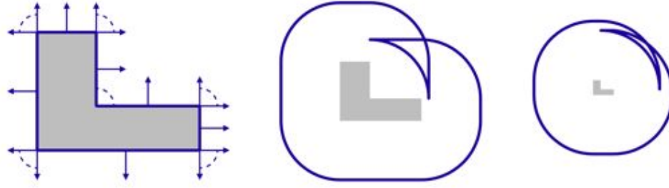
FIGURE 7.12. On the left, we show a nonconvex polygon in gray with its normal field indicated in blue. In the middle, we show the polygon's \frac{1}{2} -Gauss offset, which self-intersects due to the polygon's concave vertex. On the right, we show the polygon's \epsilon -Gauss offset as \epsilon goes to zero. The offset approximates a circle, but it has folds with patches where geodesically distant points with similar normals map to nearby points under the Gauss offset.
