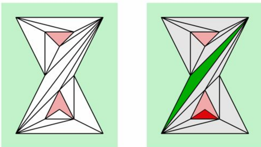
FIGURE 9.1. On the left, we show a triangulation of the space between R and G . On the right, we shade gray the triangles whose vertices lie on the boundaries of both R and G . We shade the triangle whose vertices lie on R red, and we shade the triangle whose vertices lie on G green.
